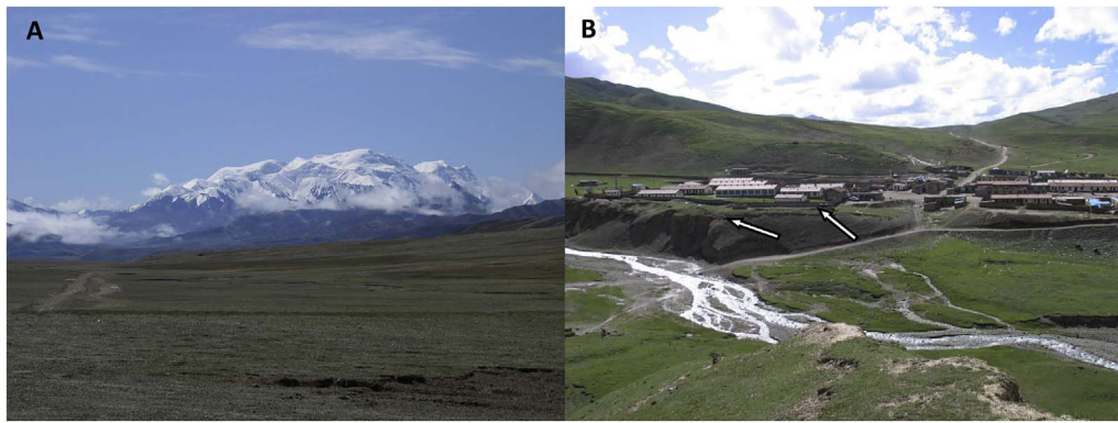
Fig. 12. (A) View of the Amnye Machen 15–20 km southeast of Xiadawu. (B) View of the Tibetan village of Xiadawu looking west showing the location of a probable late Upper Paleolithic earth oven near the village (left arrow). Note that the feature lies at a point where a meander of the small stream is eroding the stream margin during periods of high flood water. The remnant of the simple hearth lies at the base of the loess 40 m downstream from the earth oven (right arrow).
